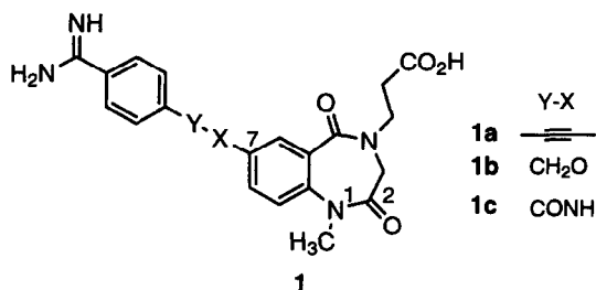
Figure 1. Benzodiazepines 1a–c .
